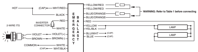
FIG R TWO (2) LAMPS WITHOUT AC BALLAST
