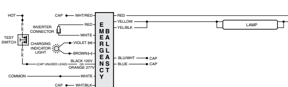
FIG 109 ONE (1) 32-215 W LAMP WITHOUT AC BALLAST
