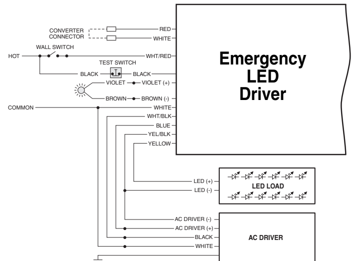
FIG B SEPARATE LED AND TEST SWITCH
