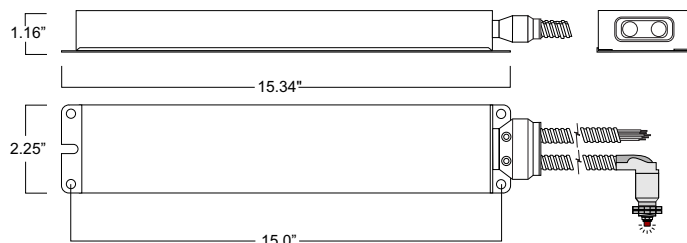
BSL310C-DF (Metal case, dual conduit) Weight: 3.80 lbs. (1.73kg) Order no. BSL310CDFM
